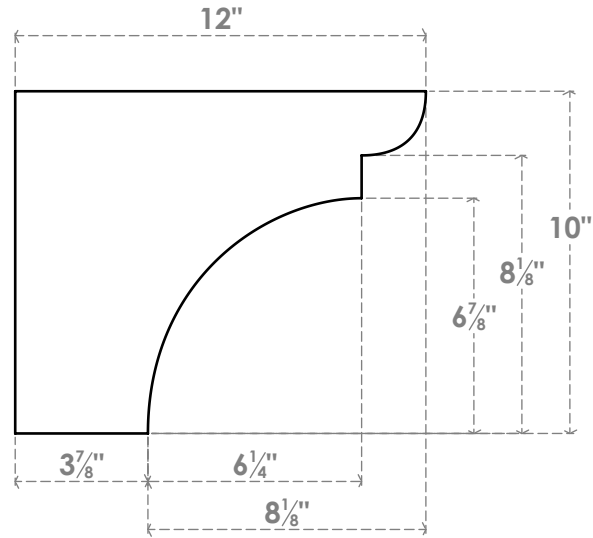
SIDE PROFILE
